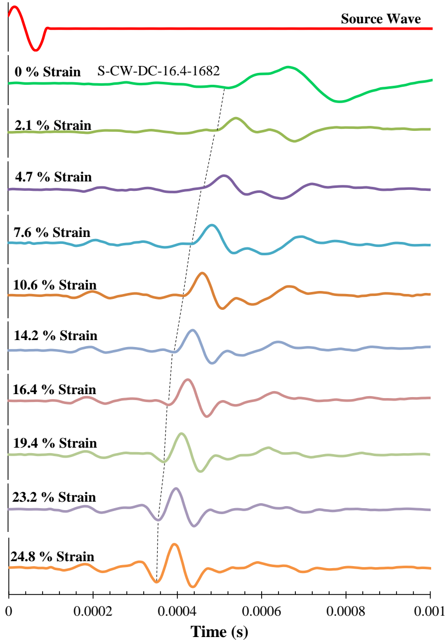
Figure 5.14 Shear (S) waves received for the DCsclay soil specimen S-CW-DC-16.4-1682, at different points of axial strain, showing the trend of characteristic point of first trough.
