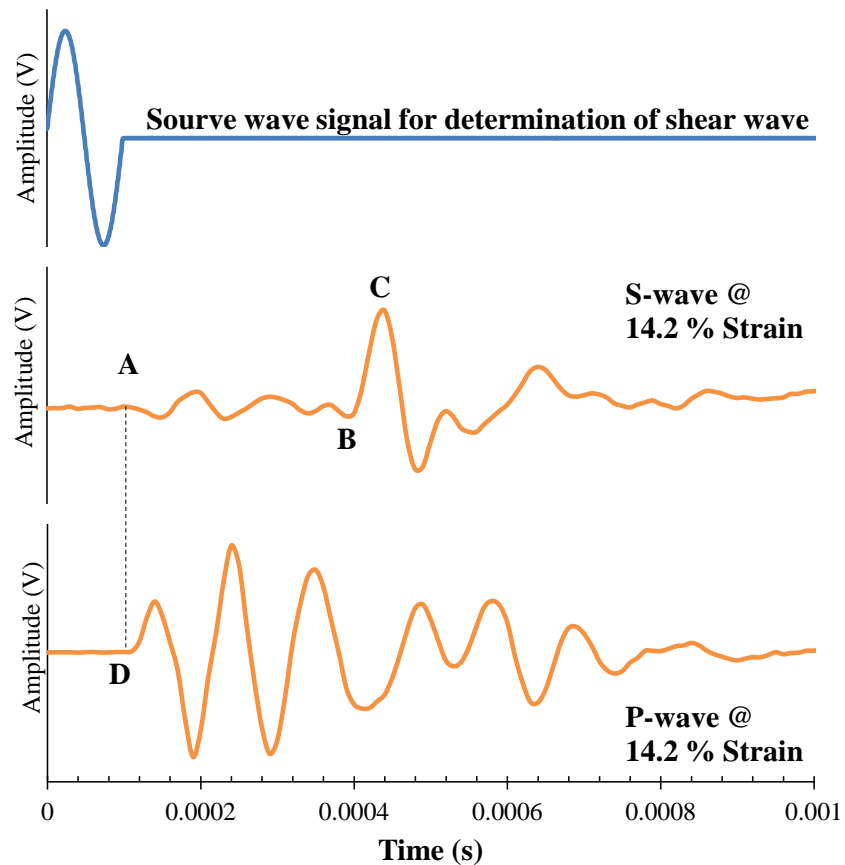
Figure 5.13 Shear (S) and compression (P) wave received for the DCsclay soil specimen under the same stress state conditions, showing the near field effect.
