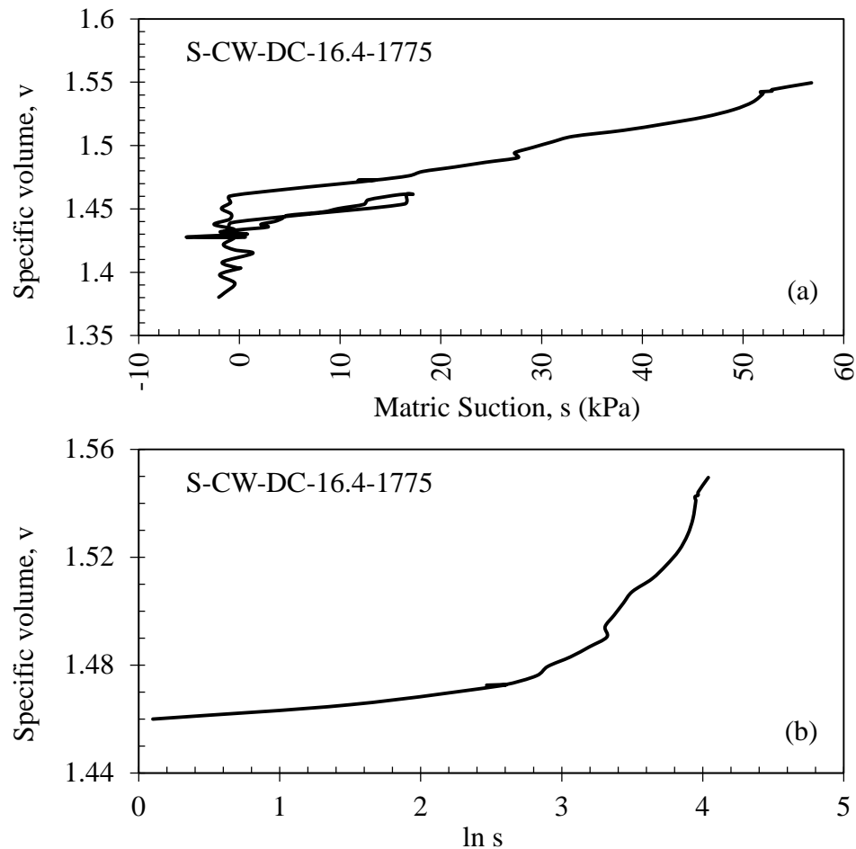
Figure 6.3 Experimental test data trends of specific volume for the DCsclay soil initially compacted to the standard Proctor maximum dry density and optimum moisture content, isotropically compressed under conditions of constant water content: (a) with respect to matric suction; (b) with respect to the natural logarithm of matric suction.
