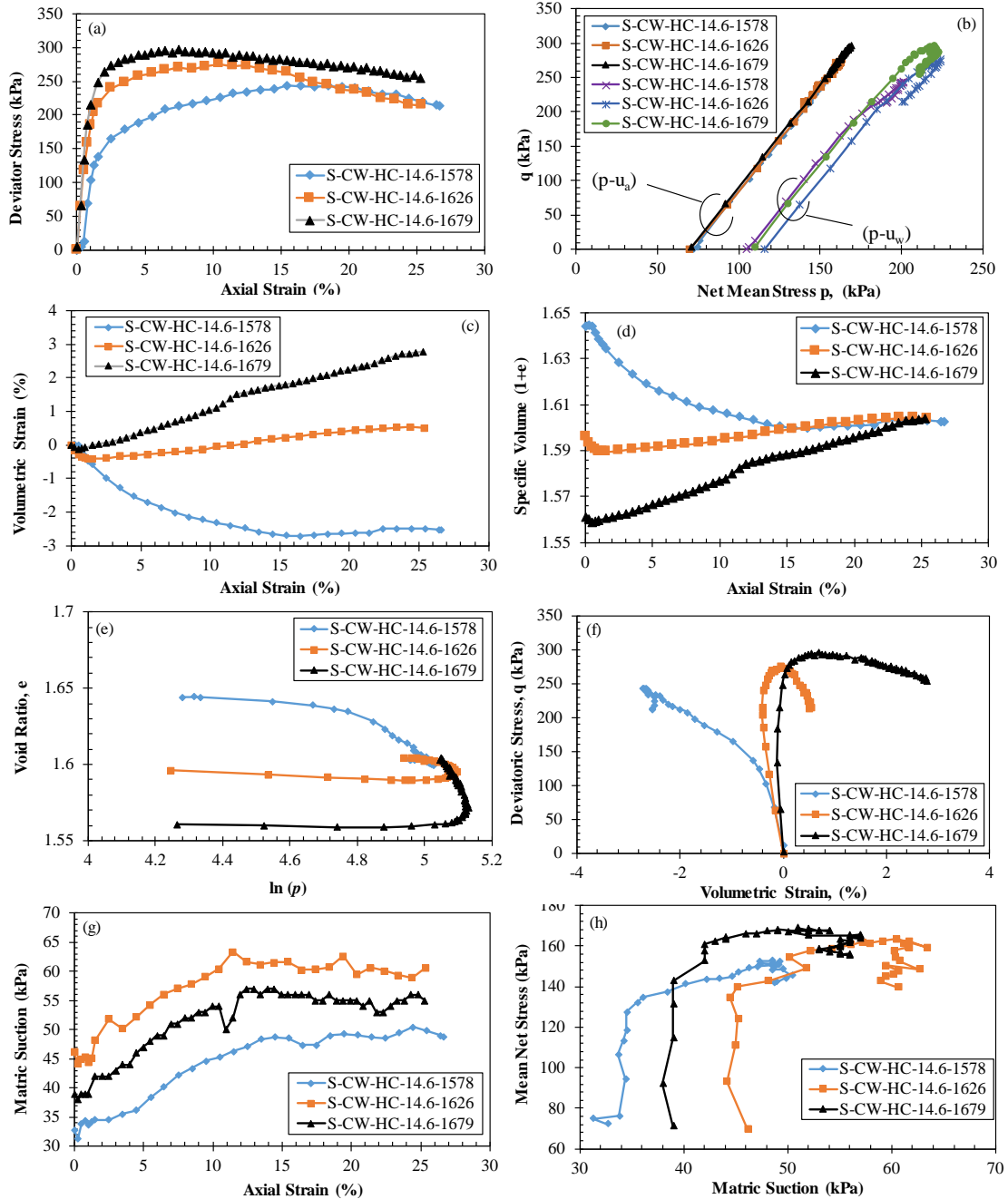
Figure H.13 Shear phase CW triaxial tests experimental data for the HC clay at different initial densities
