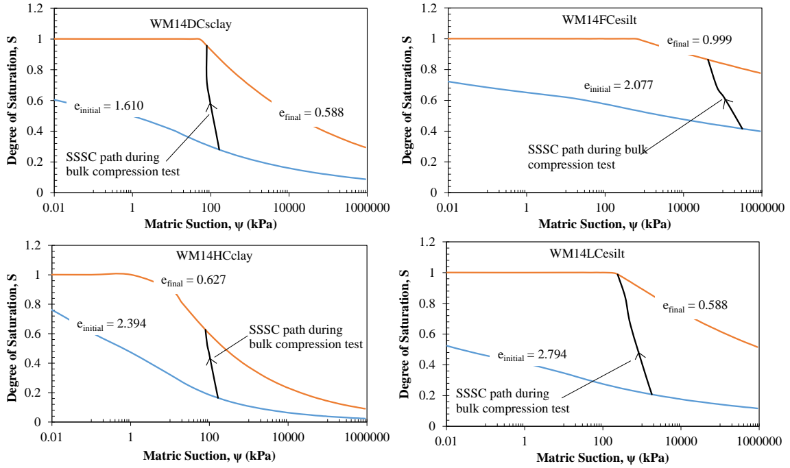
Figure G.1 SSSC paths determined from estimated matric suctions using the ZhouSWCCshiffforsuction VBA Code.
