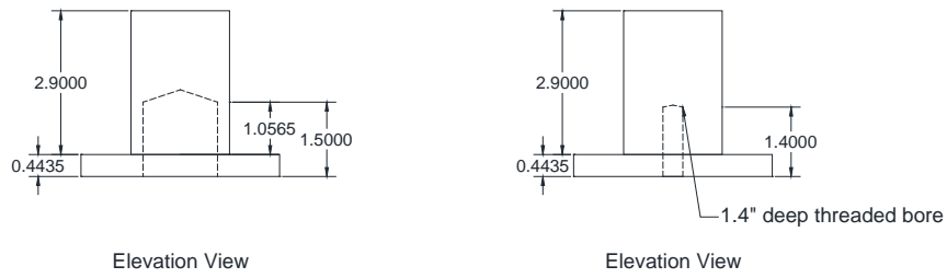
Figure C.47 Details of the top and bottom pistons of the compaction split mold for fabricating the unsaturated triaxial and soil-water retention test specimens.
