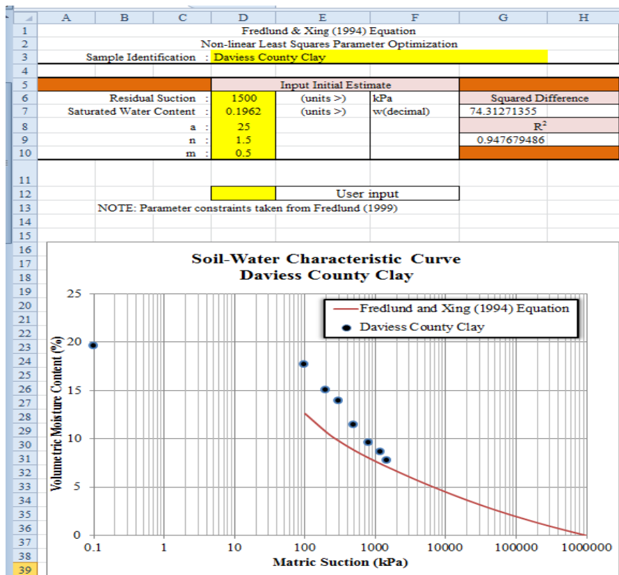
Figure D.1. General Layout of Fredlund and Xing (1994) Optimizer in Microsoft Excel with initial parameter estimates.
