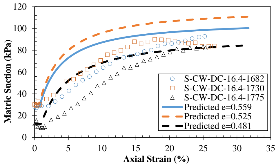
Figure 7.28 Predicted matric suction stress with axial strain response in comparison with the experimental response for the DCsclay soil specimens at different initial densities under conditions of constant-water content.
